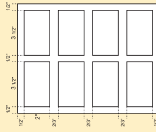
Cutting mode #3 Double cut
