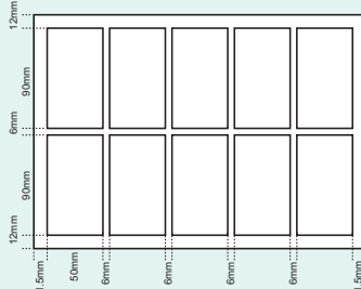
Cutting mode #5 Double cut
