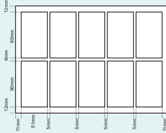
Cutting mode #4 Double cut
