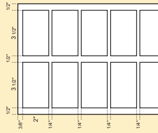
Cutting mode #5 Double cut
