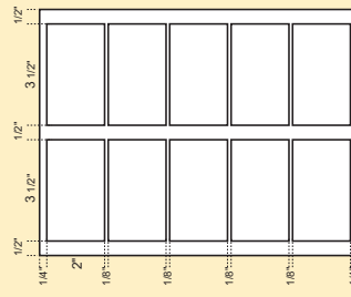
Cutting mode #2 Double cut
