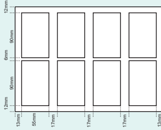
Cutting mode #3 Double cut
