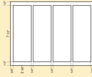
Cutting mode #4 Double cut
